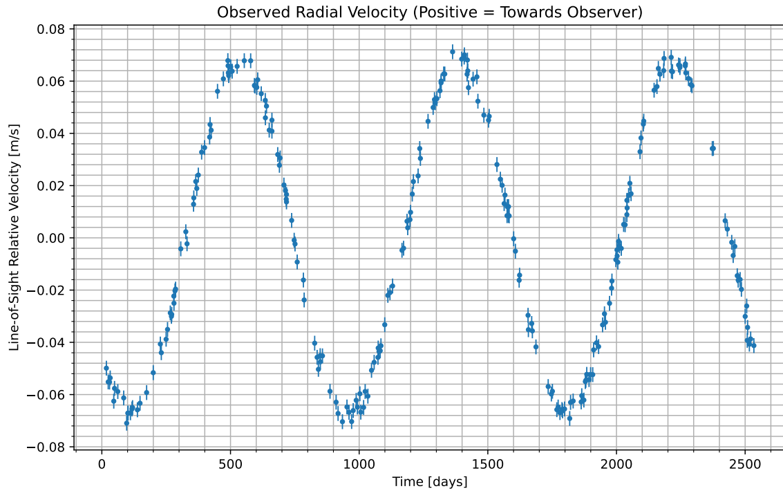
Figure 1: We have isolated the radial velocity of the host star due to the candidate planet. Data begins at UTC 2092-04-17/13:20. Positive values indicate the velocity at which the star is moving towards us; negative indicate the velocity at which it is moving away.
