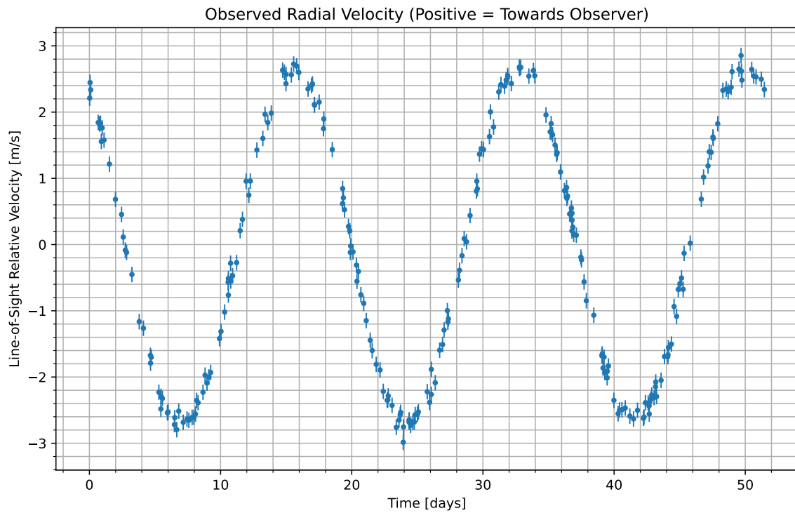
Figure 1: We have isolated the radial velocity of the host star due to the candidate planet. Data begins at UTC 2077-05-04/15:54. Positive values indicate the velocity at which the star is moving towards us; negative indicate the velocity at which it is moving away.
