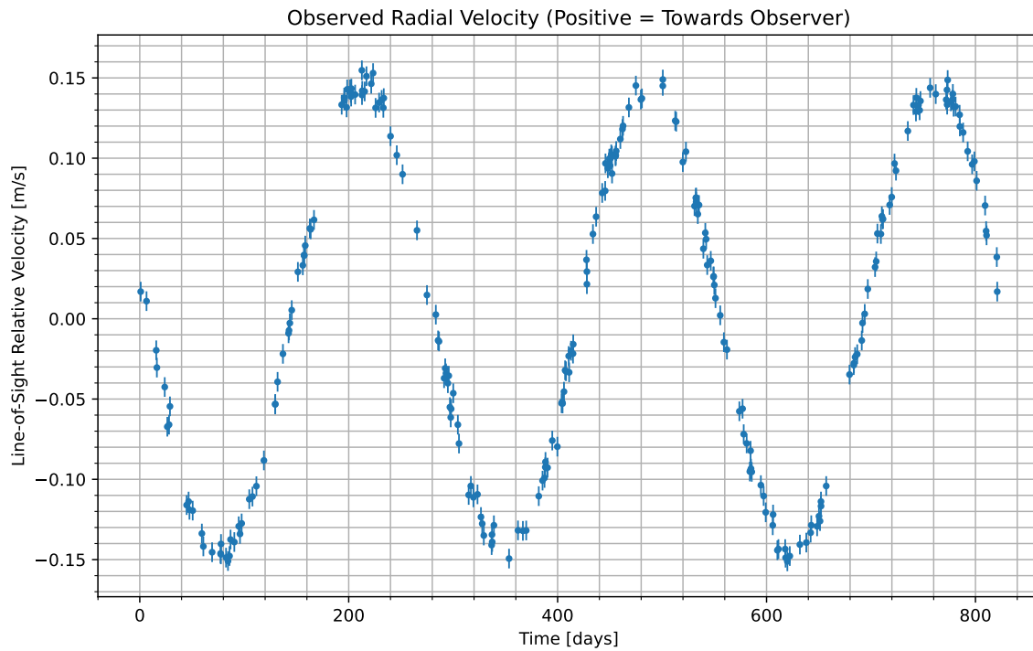
Figure 1: We have isolated the radial velocity of the host star due to the candidate planet. Data begins at UTC 2072-10-27/23:36. Positive values indicate the velocity at which the star is moving towards us; negative indicate the velocity at which it is moving away.
