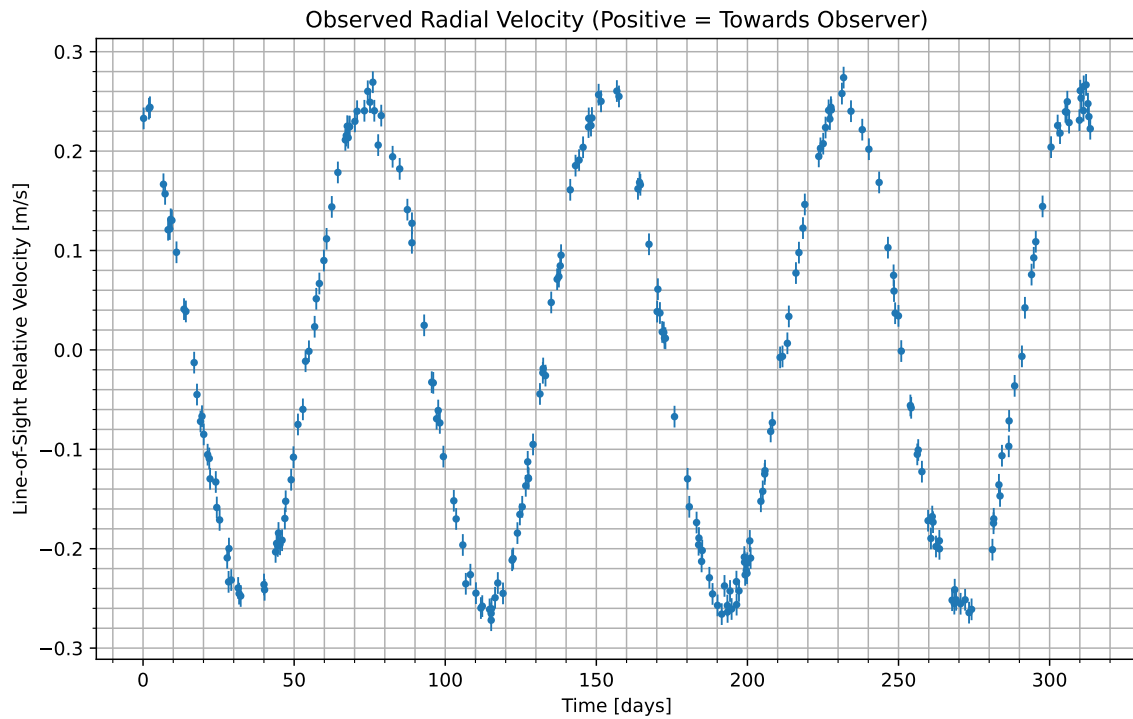
Figure 1: We have isolated the radial velocity of the host star due to the candidate planet. Data begins at UTC 2092-12-31/16:00. Positive values indicate the velocity at which the star is moving towards us; negative indicate the velocity at which it is moving away.
