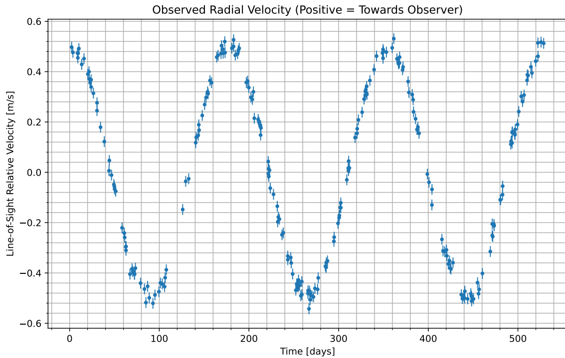
Figure 1: We have isolated the radial velocity of the host star due to the candidate planet. Data begins at UTC 2091-07-02/17:54. Positive values indicate the velocity at which the star is moving towards us; negative indicate the velocity at which it is moving away.
