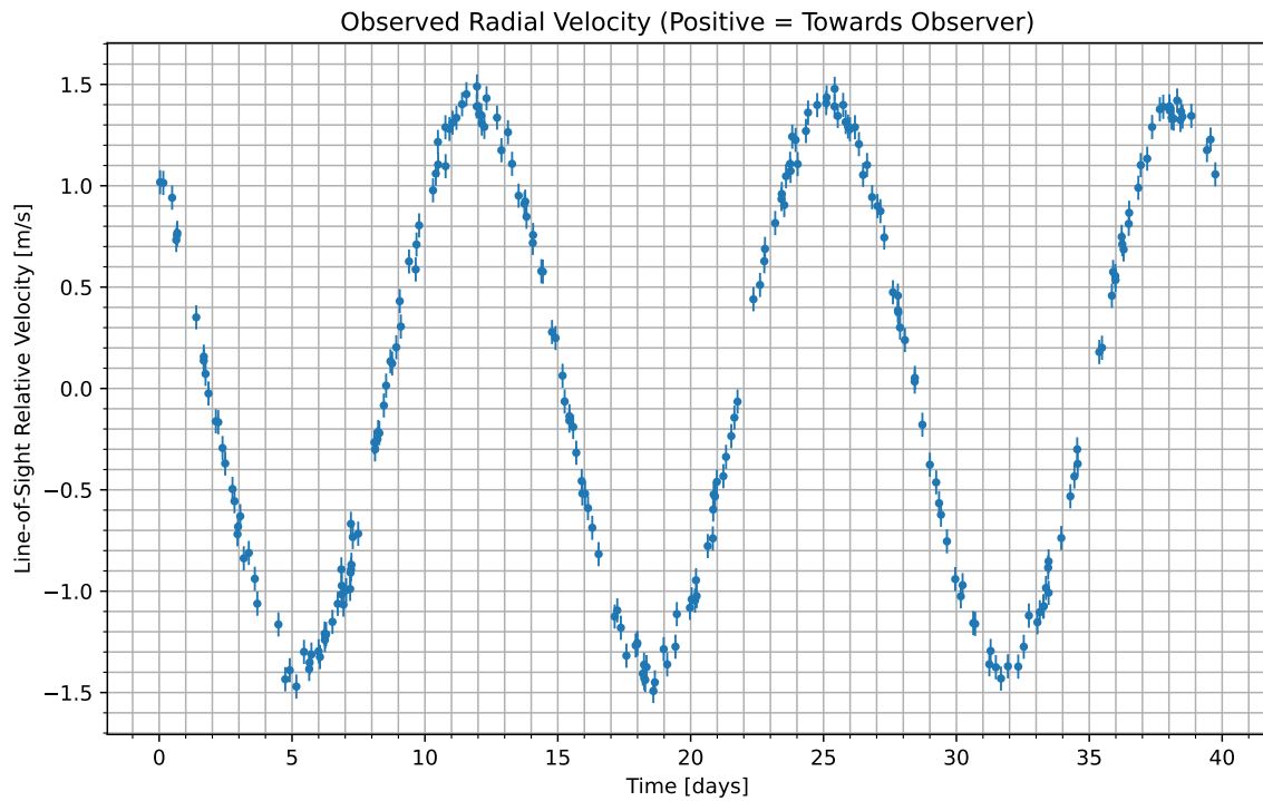
Figure 1: We have isolated the radial velocity of the host star due to the candidate planet. Data begins at UTC 2080-11-15/01:09. Positive values indicate the velocity at which the star is moving towards us; negative indicate the velocity at which it is moving away.
