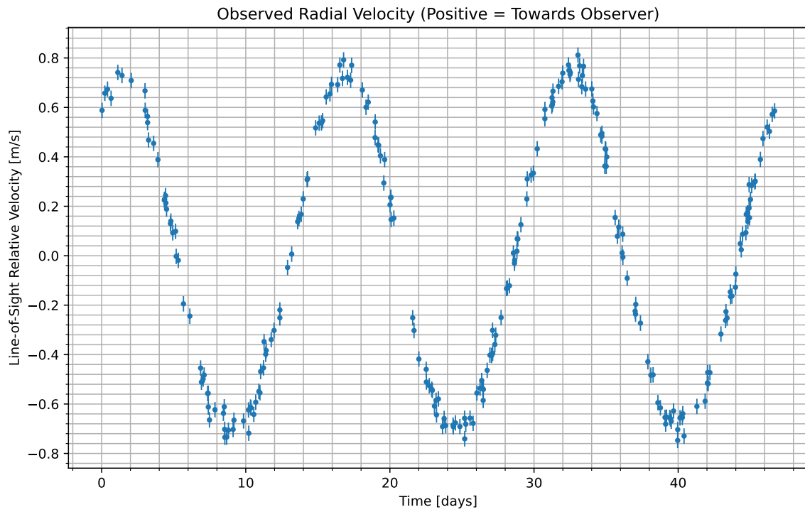
Figure 1: We have isolated the radial velocity of the host star due to the candidate planet. Data begins at UTC 2079-11-26/01:37. Positive values indicate the velocity at which the star is moving towards us; negative indicate the velocity at which it is moving away.
