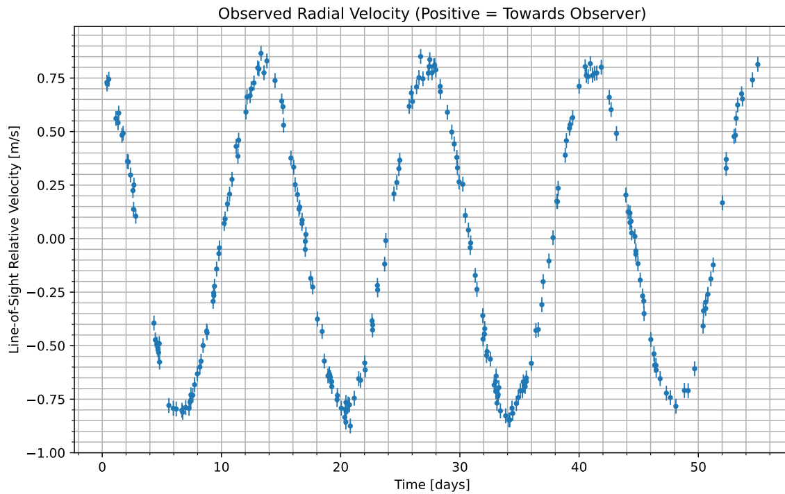
Figure 1: We have isolated the radial velocity of the host star due to the candidate planet. Data begins at UTC 2095-10-02/12:37. Positive values indicate the velocity at which the star is moving towards us; negative indicate the velocity at which it is moving away.
