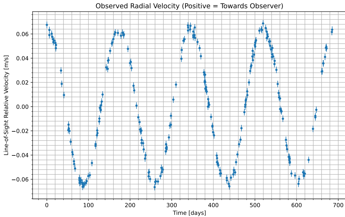
Figure 1: We have isolated the radial velocity of the host star due to the candidate planet. Data begins at UTC 2086-07-14/02:19. Positive values indicate the velocity at which the star is moving towards us; negative indicate the velocity at which it is moving away.
