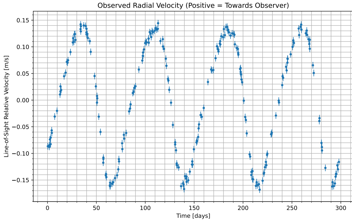
Figure 1: We have isolated the radial velocity of the host star due to the candidate planet. Data begins at UTC 2073-10-20/13:53. Positive values indicate the velocity at which the star is moving towards us; negative indicate the velocity at which it is moving away.
