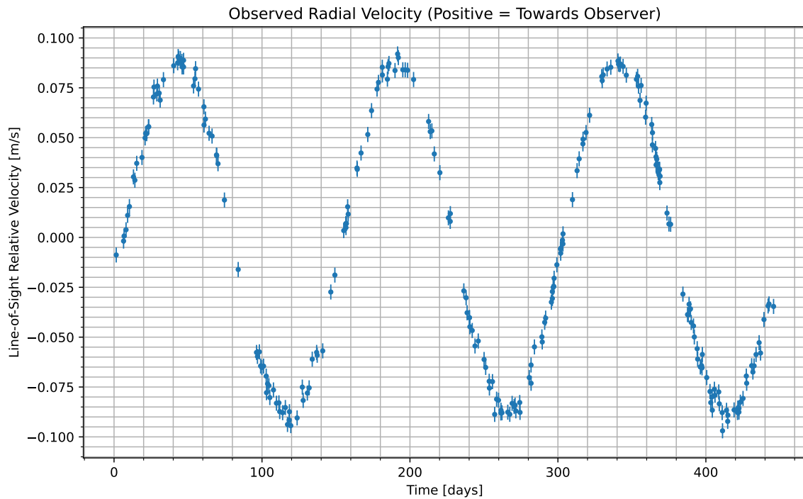
Figure 1: We have isolated the radial velocity of the host star due to the candidate planet. Data begins at UTC 2078-04-03/19:01. Positive values indicate the velocity at which the star is moving towards us; negative indicate the velocity at which it is moving away.
