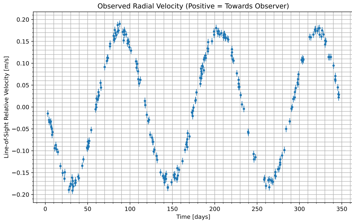
Figure 1: We have isolated the radial velocity of the host star due to the candidate planet. Data begins at UTC 2090-02-28/10:23. Positive values indicate the velocity at which the star is moving towards us; negative indicate the velocity at which it is moving away.
