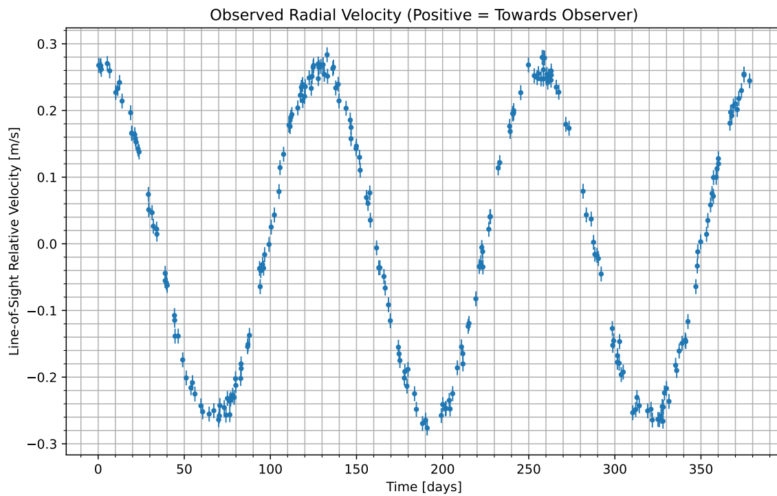
Figure 1: We have isolated the radial velocity of the host star due to the candidate planet. Data begins at UTC 2098-05-17/08:57. Positive values indicate the velocity at which the star is moving towards us; negative indicate the velocity at which it is moving away.
