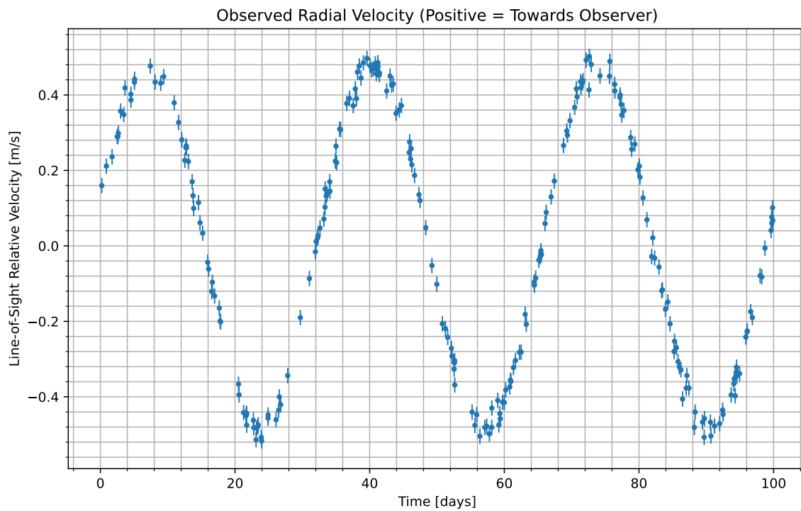
Figure 1: We have isolated the radial velocity of the host star due to the candidate planet. Data begins at UTC 2072-12-09/17:08. Positive values indicate the velocity at which the star is moving towards us; negative indicate the velocity at which it is moving away.
