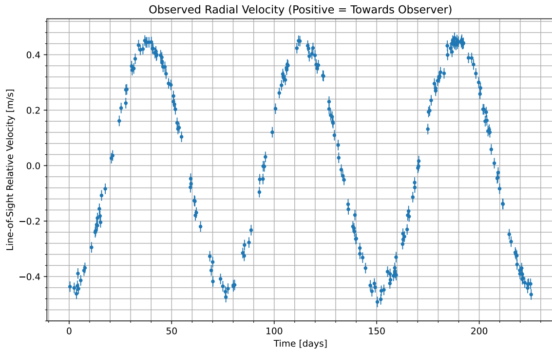
Figure 1: We have isolated the radial velocity of the host star due to the candidate planet. Data begins at UTC 2090-02-26/06:42. Positive values indicate the velocity at which the star is moving towards us; negative indicate the velocity at which it is moving away.
