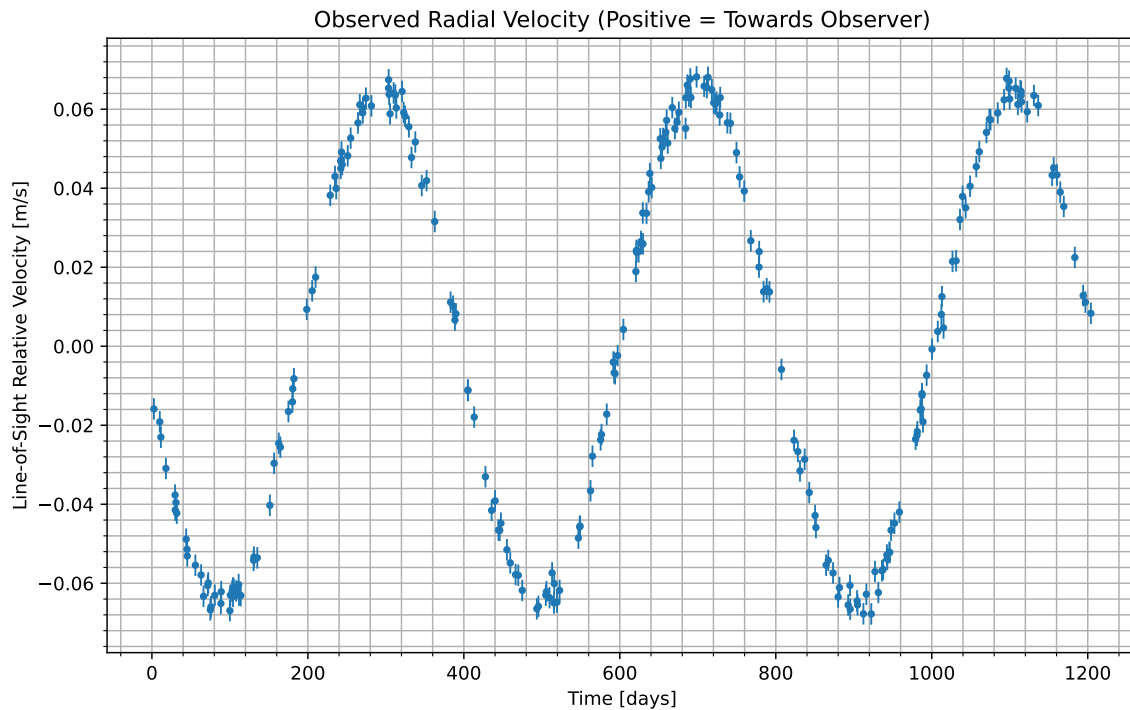
Figure 1: We have isolated the radial velocity of the host star due to the candidate planet. Data begins at UTC 2075-08-02/18:42. Positive values indicate the velocity at which the star is moving towards us; negative indicate the velocity at which it is moving away.
