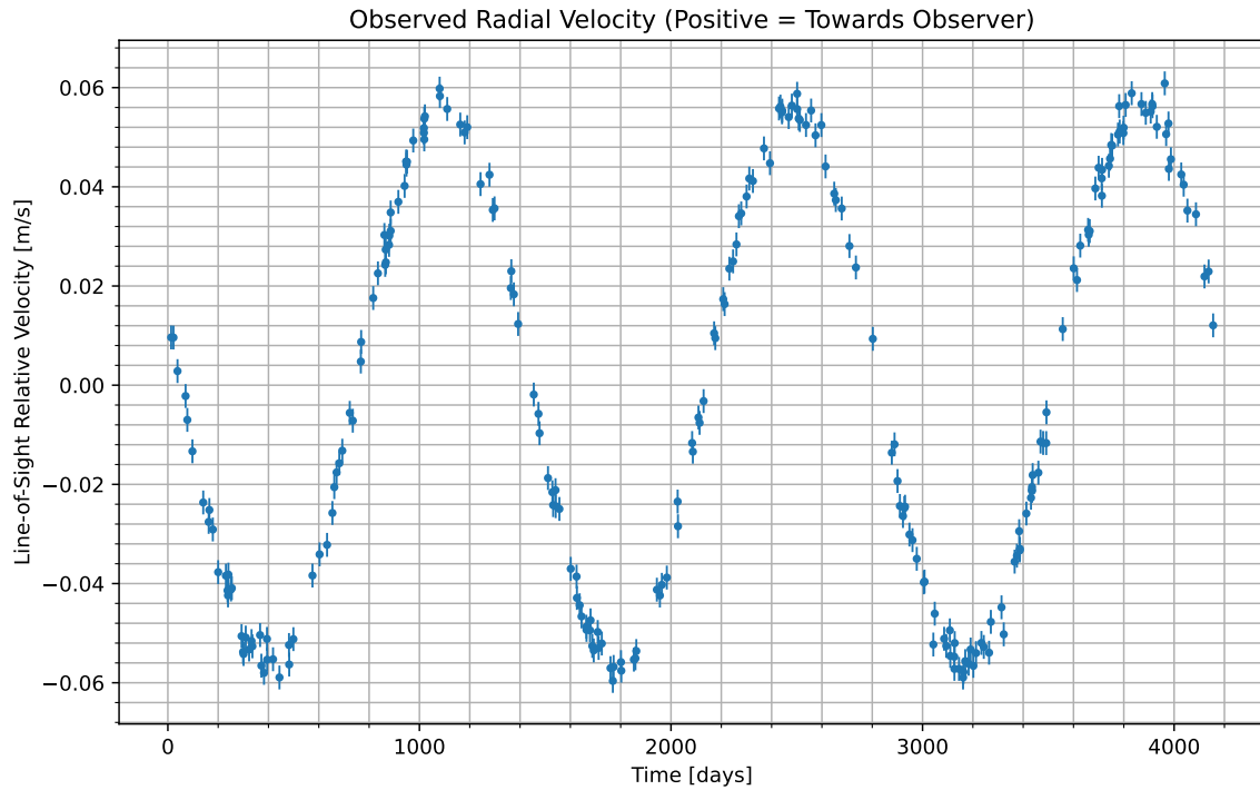
Figure 1: We have isolated the radial velocity of the host star due to the candidate planet. Data begins at UTC 2068-08-08/04:19. Positive values indicate the velocity at which the star is moving towards us; negative indicate the velocity at which it is moving away.
