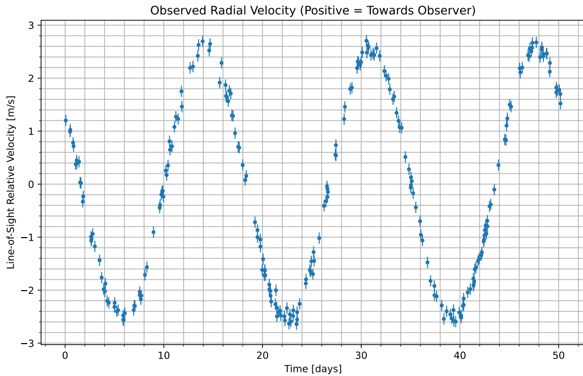
Figure 1: We have isolated the radial velocity of the host star due to the candidate planet. Data begins at UTC 2096-02-08/18:10. Positive values indicate the velocity at which the star is moving towards us; negative indicate the velocity at which it is moving away.
