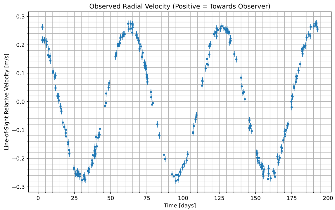
Figure 1: We have isolated the radial velocity of the host star due to the candidate planet. Data begins at UTC 2080-10-15/03:57. Positive values indicate the velocity at which the star is moving towards us; negative indicate the velocity at which it is moving away.
