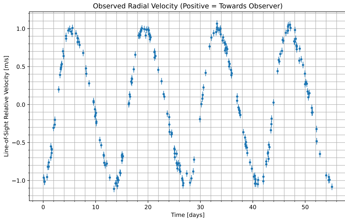
Figure 1: We have isolated the radial velocity of the host star due to the candidate planet. Data begins at UTC 2080-04-06/07:07. Positive values indicate the velocity at which the star is moving towards us; negative indicate the velocity at which it is moving away.
