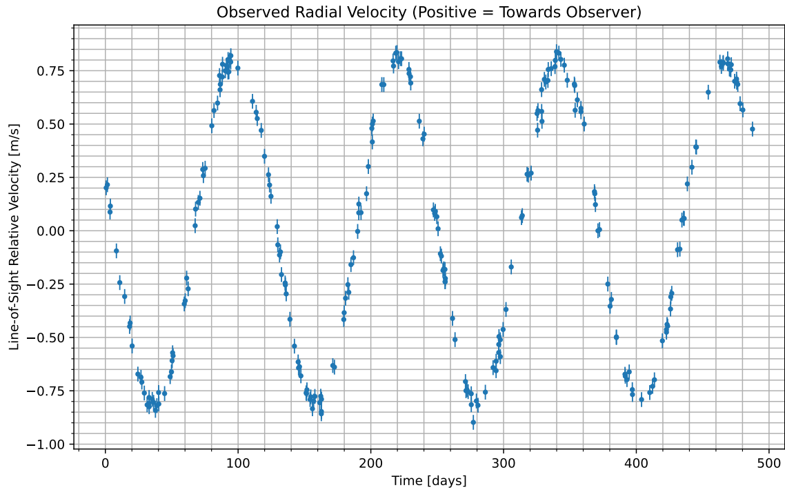
Figure 1: We have isolated the radial velocity of the host star due to the candidate planet. Data begins at UTC 2098-01-08/14:27. Positive values indicate the velocity at which the star is moving towards us; negative indicate the velocity at which it is moving away.
