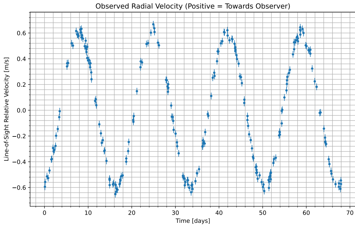
Figure 1: We have isolated the radial velocity of the host star due to the candidate planet. Data begins at UTC 2094-05-09/12:01. Positive values indicate the velocity at which the star is moving towards us; negative indicate the velocity at which it is moving away.
