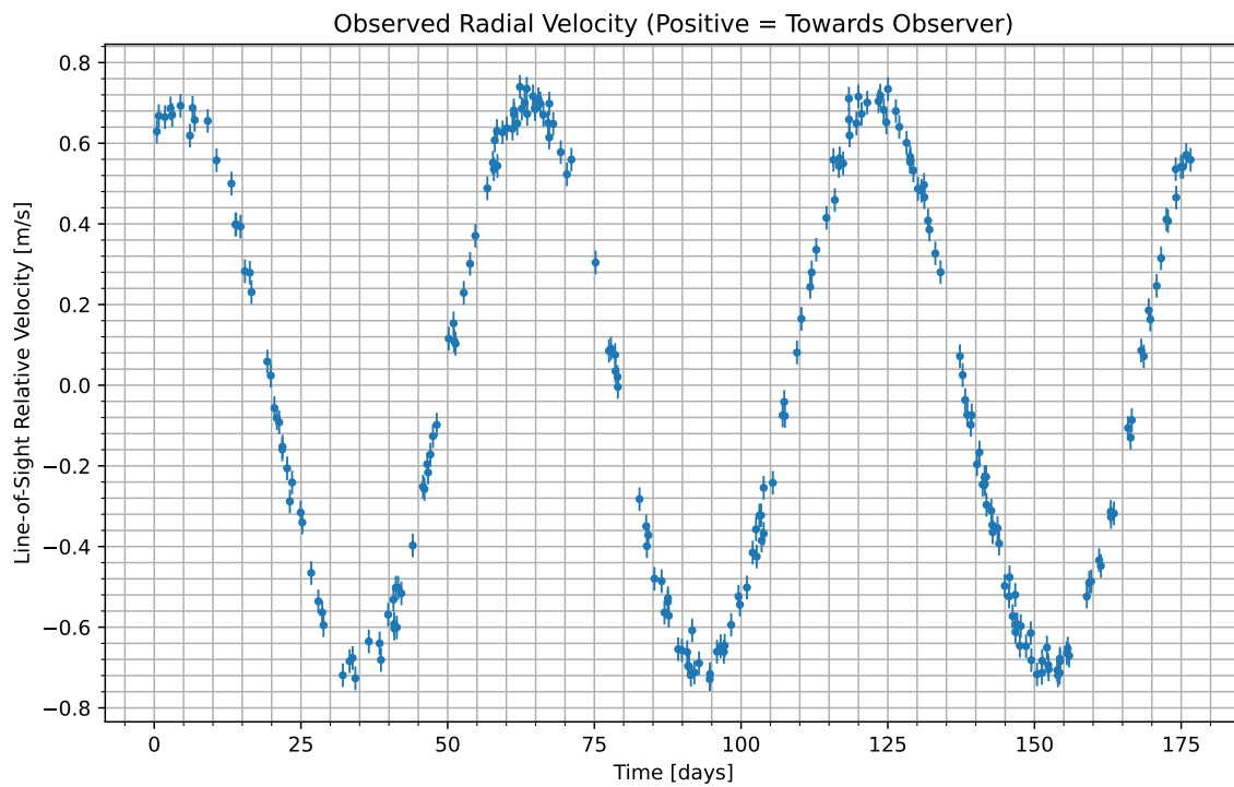
Figure 1: We have isolated the radial velocity of the host star due to the candidate planet. Data begins at UTC 2094-09-15/04:32. Positive values indicate the velocity at which the star is moving towards us; negative indicate the velocity at which it is moving away.
