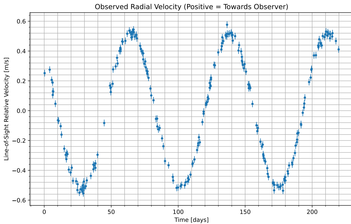
Figure 1: We have isolated the radial velocity of the host star due to the candidate planet. Data begins at UTC 2086-06-25/18:03. Positive values indicate the velocity at which the star is moving towards us; negative indicate the velocity at which it is moving away.
