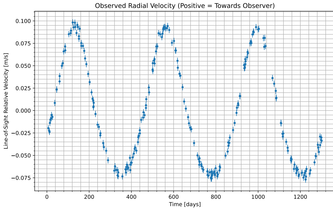
Figure 1: We have isolated the radial velocity of the host star due to the candidate planet. Data begins at UTC 2079-04-11/10:30. Positive values indicate the velocity at which the star is moving towards us; negative indicate the velocity at which it is moving away.
