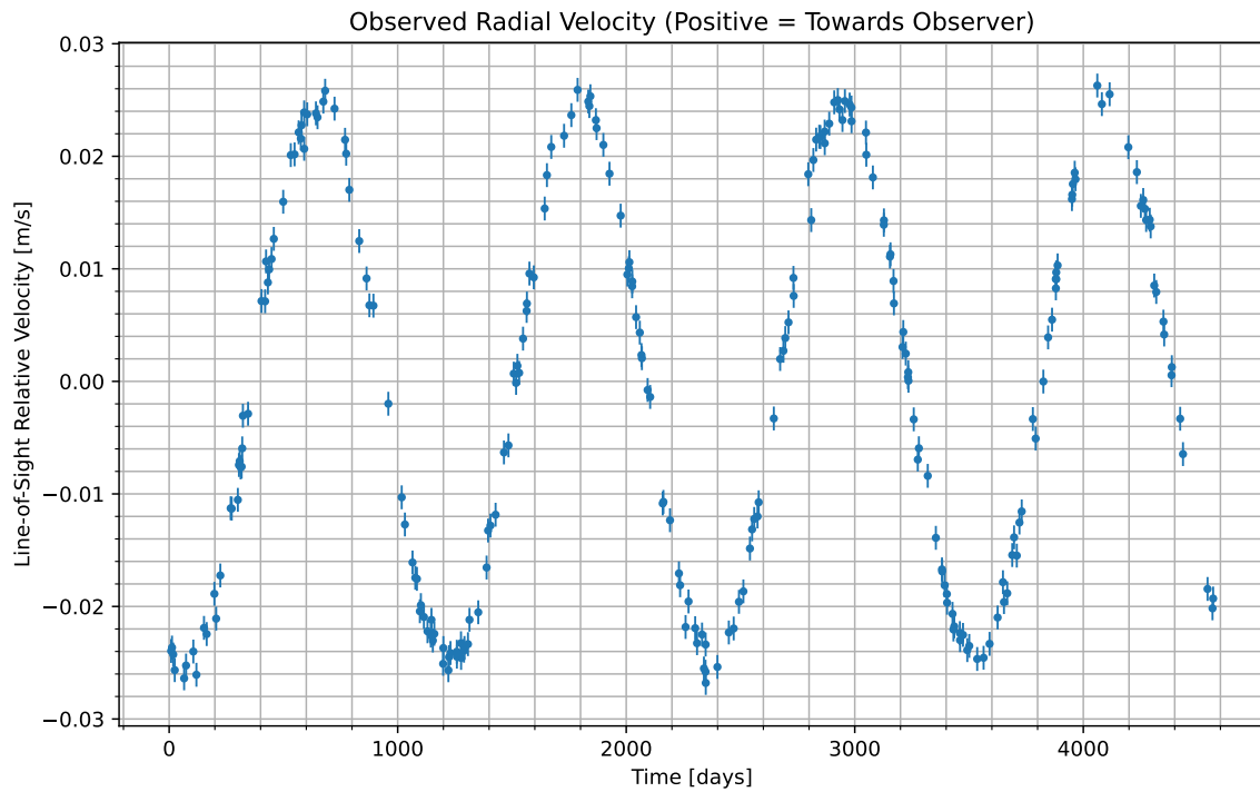
Figure 1: We have isolated the radial velocity of the host star due to the candidate planet. Data begins at UTC 2068-10-30/01:24. Positive values indicate the velocity at which the star is moving towards us; negative indicate the velocity at which it is moving away.
