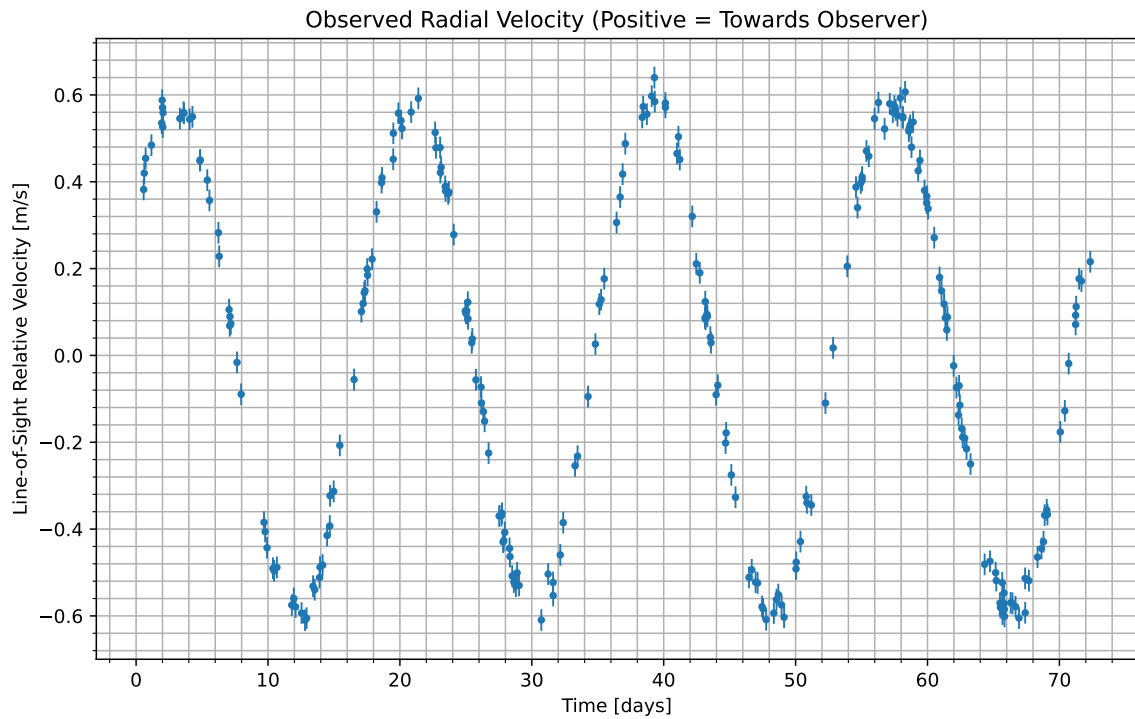
Figure 1: We have isolated the radial velocity of the host star due to the candidate planet. Data begins at UTC 2075-05-07/20:50. Positive values indicate the velocity at which the star is moving towards us; negative indicate the velocity at which it is moving away.
