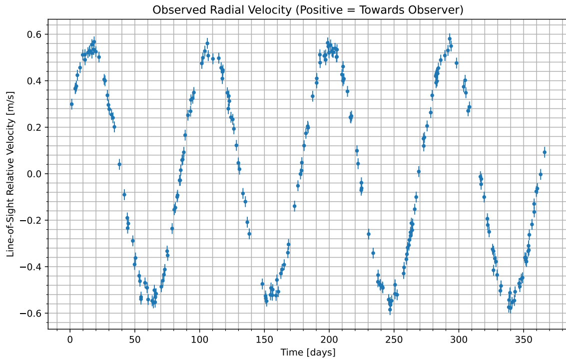
Figure 1: We have isolated the radial velocity of the host star due to the candidate planet. Data begins at UTC 2094-04-09/14:58. Positive values indicate the velocity at which the star is moving towards us; negative indicate the velocity at which it is moving away.
