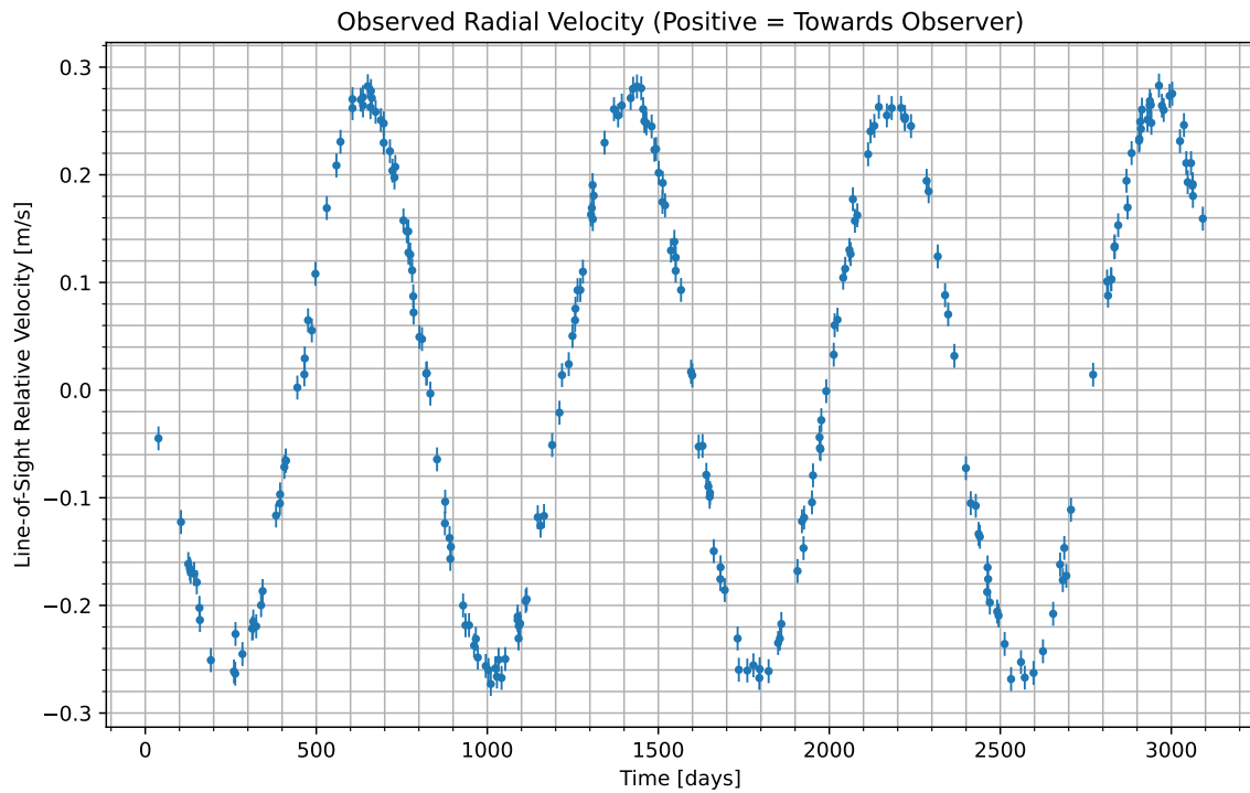
Figure 1: We have isolated the radial velocity of the host star due to the candidate planet. Data begins at UTC 2077-12-02/07:30. Positive values indicate the velocity at which the star is moving towards us; negative indicate the velocity at which it is moving away.
