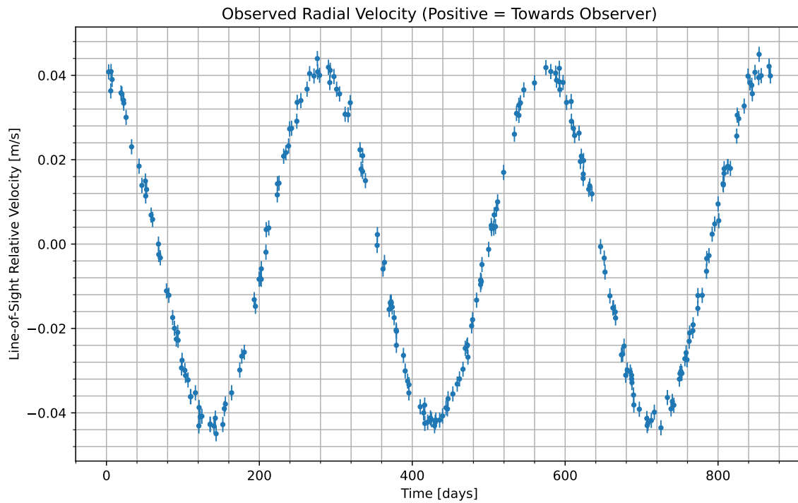
Figure 1: We have isolated the radial velocity of the host star due to the candidate planet. Data begins at UTC 2068-05-21/19:05. Positive values indicate the velocity at which the star is moving towards us; negative indicate the velocity at which it is moving away.
