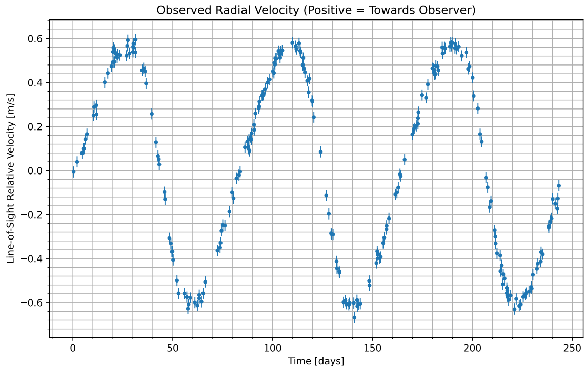
Figure 1: We have isolated the radial velocity of the host star due to the candidate planet. Data begins at UTC 2073-12-14/02:53. Positive values indicate the velocity at which the star is moving towards us; negative indicate the velocity at which it is moving away.
