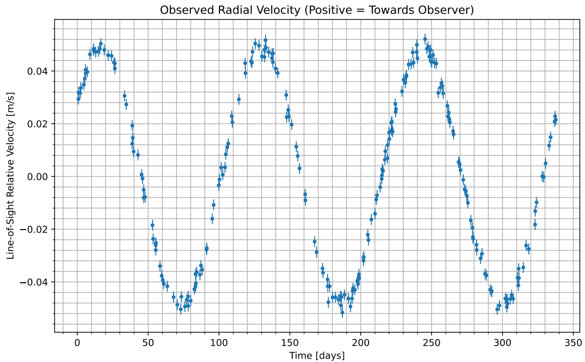
Figure 1: We have isolated the radial velocity of the host star due to the candidate planet. Data begins at UTC 2087-07-20/23:37. Positive values indicate the velocity at which the star is moving towards us; negative indicate the velocity at which it is moving away.
