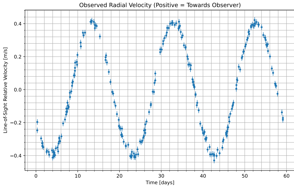
Figure 1: We have isolated the radial velocity of the host star due to the candidate planet. Data begins at UTC 2075-03-27/08:11. Positive values indicate the velocity at which the star is moving towards us; negative indicate the velocity at which it is moving away.
