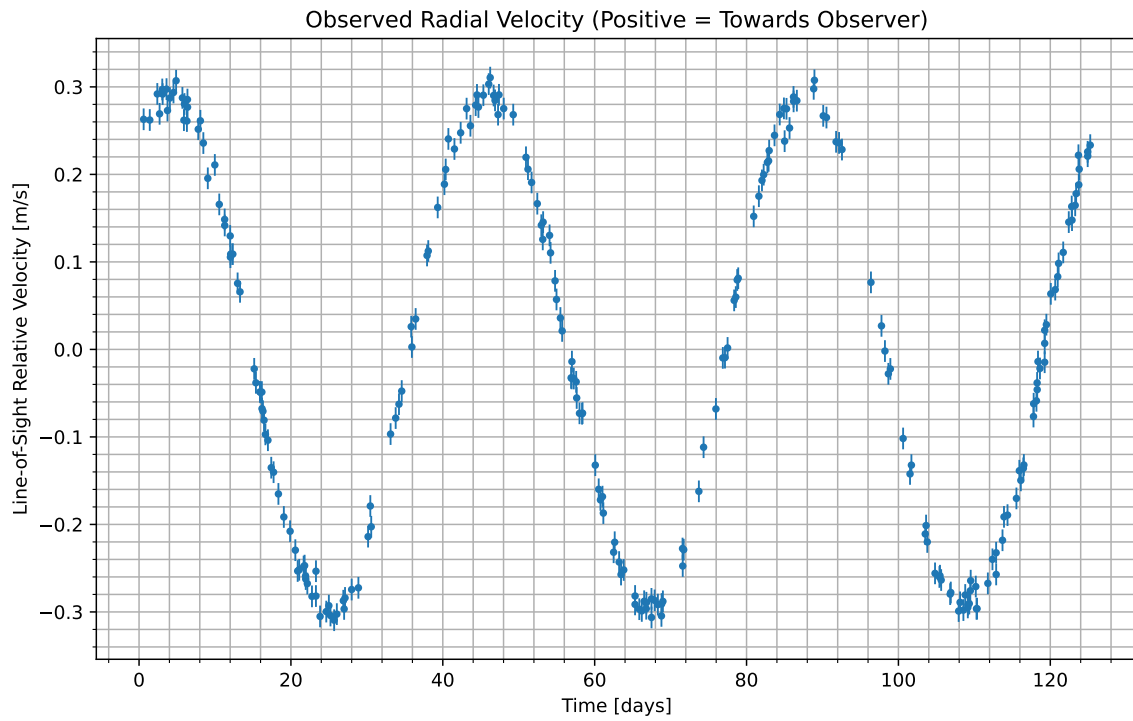
Figure 1: We have isolated the radial velocity of the host star due to the candidate planet. Data begins at UTC 2081-11-07/20:37. Positive values indicate the velocity at which the star is moving towards us; negative indicate the velocity at which it is moving away.
