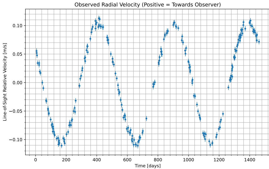
Figure 1: We have isolated the radial velocity of the host star due to the candidate planet. Data begins at UTC 2075-09-22/22:11. Positive values indicate the velocity at which the star is moving towards us; negative indicate the velocity at which it is moving away.
