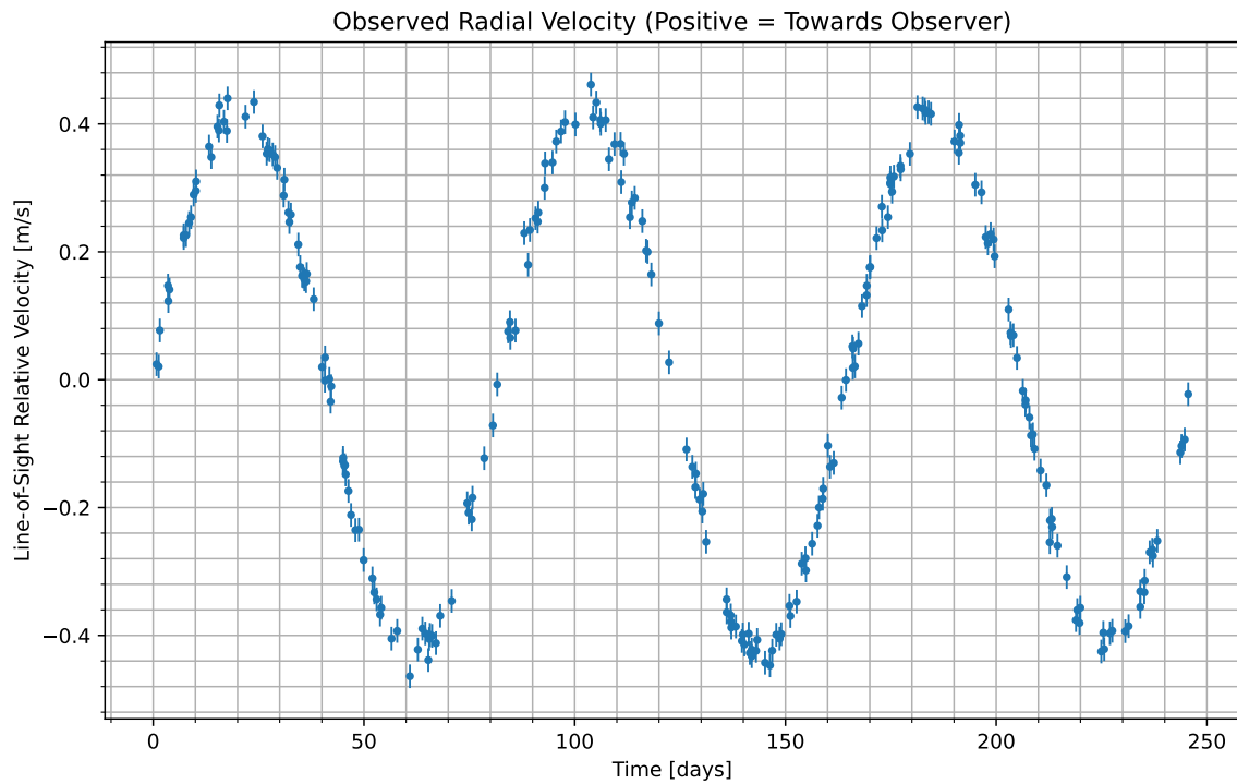
Figure 1: We have isolated the radial velocity of the host star due to the candidate planet. Data begins at UTC 2080-03-13/09:29. Positive values indicate the velocity at which the star is moving towards us; negative indicate the velocity at which it is moving away.
