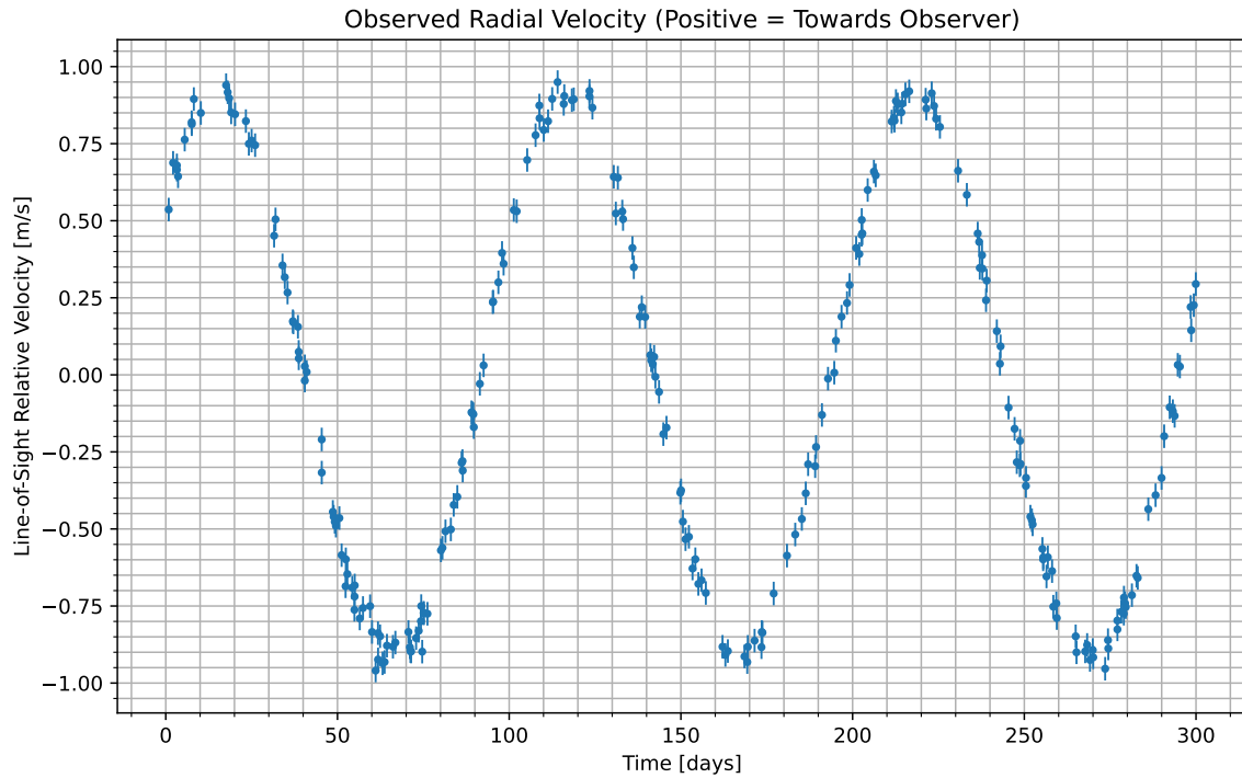
Figure 1: We have isolated the radial velocity of the host star due to the candidate planet. Data begins at UTC 2078-08-17/09:05. Positive values indicate the velocity at which the star is moving towards us; negative indicate the velocity at which it is moving away.
