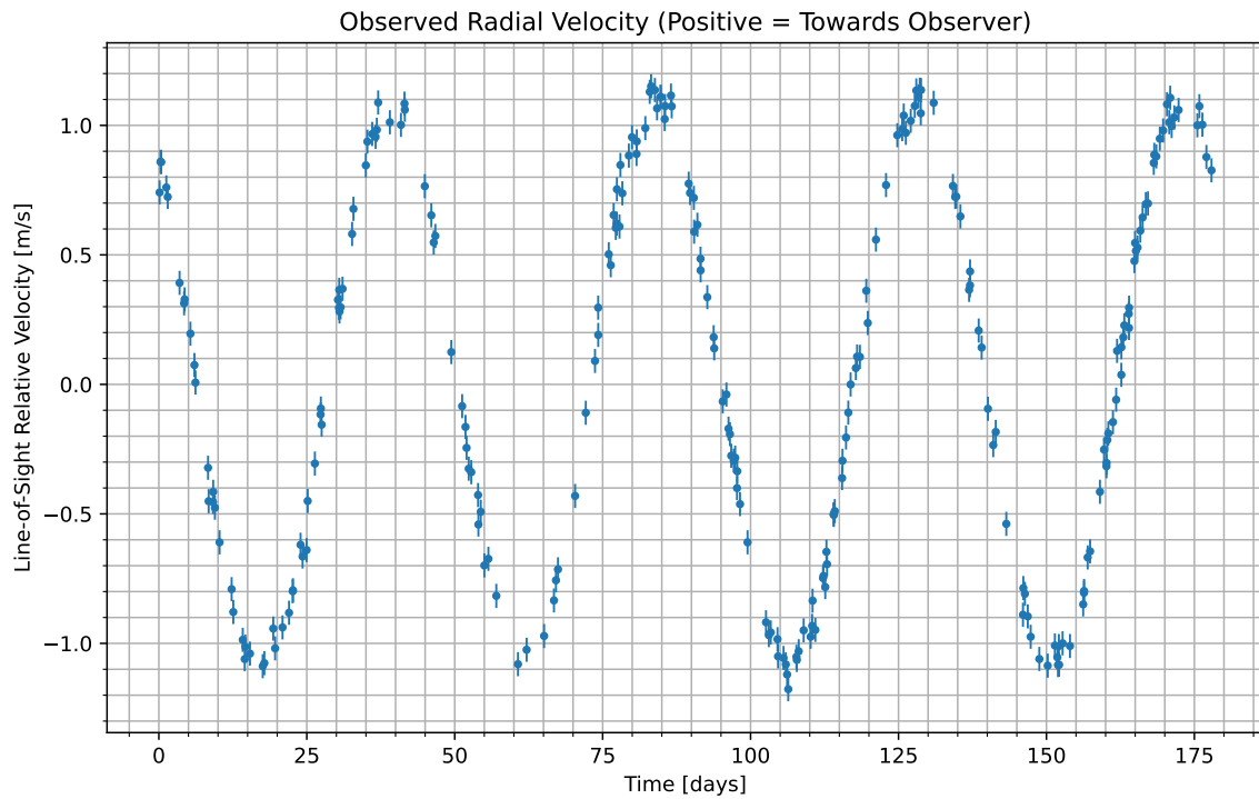
Figure 1: We have isolated the radial velocity of the host star due to the candidate planet. Data begins at UTC 2071-11-29/18:11. Positive values indicate the velocity at which the star is moving towards us; negative indicate the velocity at which it is moving away.
