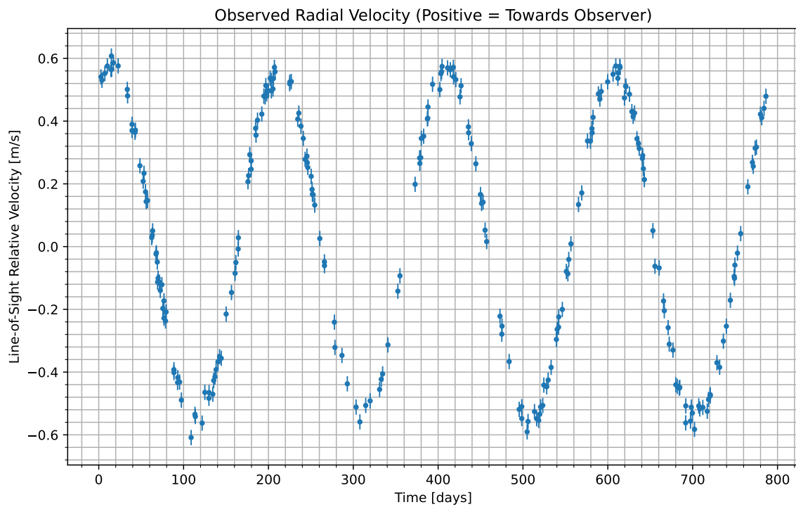
Figure 1: We have isolated the radial velocity of the host star due to the candidate planet. Data begins at UTC 2078-04-28/03:45. Positive values indicate the velocity at which the star is moving towards us; negative indicate the velocity at which it is moving away.
