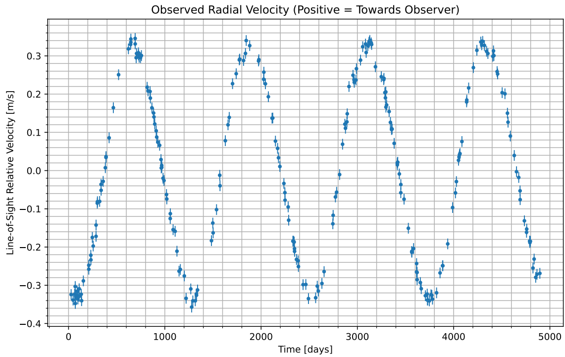
Figure 1: We have isolated the radial velocity of the host star due to the candidate planet. Data begins at UTC 2071-03-07/02:53. Positive values indicate the velocity at which the star is moving towards us; negative indicate the velocity at which it is moving away.
