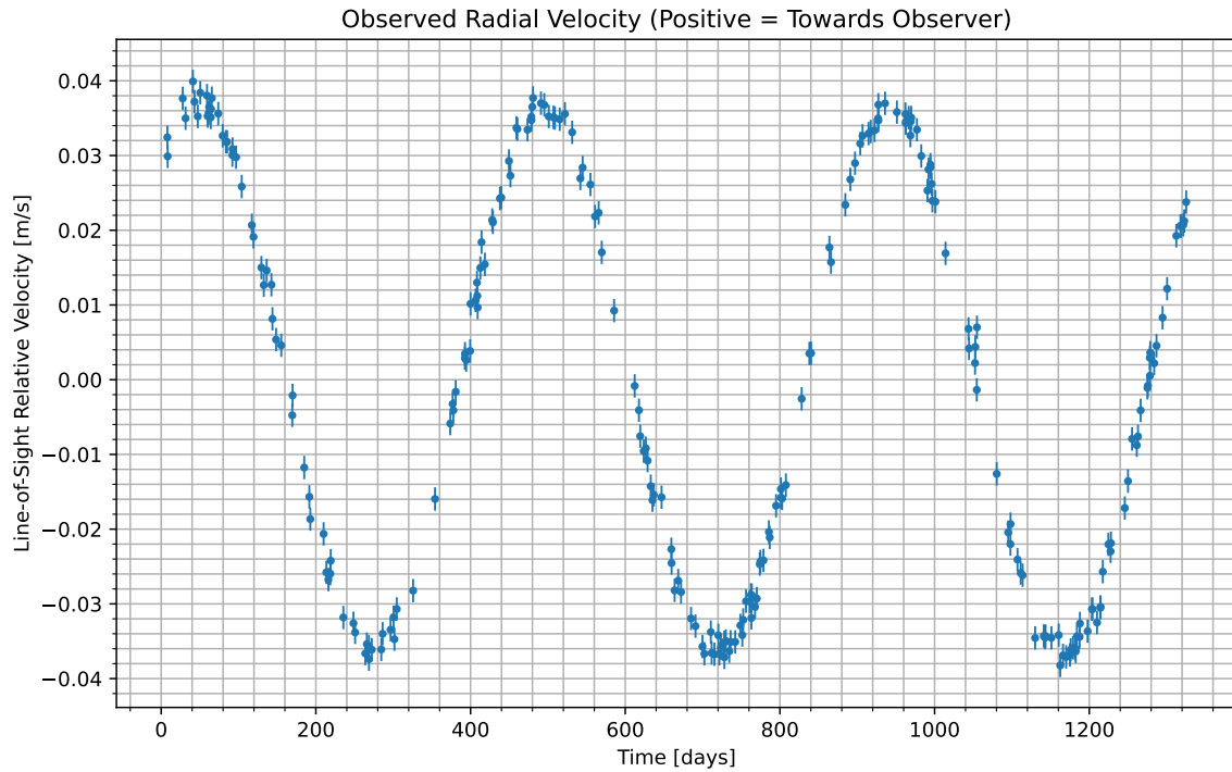
Figure 1: We have isolated the radial velocity of the host star due to the candidate planet. Data begins at UTC 2092-01-14/05:11. Positive values indicate the velocity at which the star is moving towards us; negative indicate the velocity at which it is moving away.
