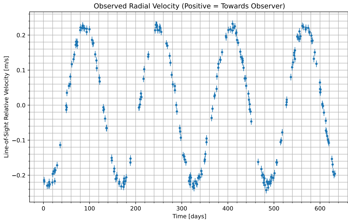
Figure 1: We have isolated the radial velocity of the host star due to the candidate planet. Data begins at UTC 2093-02-10/00:35. Positive values indicate the velocity at which the star is moving towards us; negative indicate the velocity at which it is moving away.
