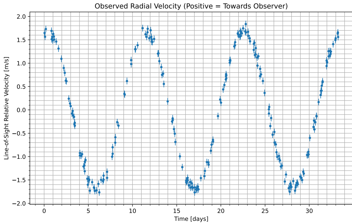
Figure 1: We have isolated the radial velocity of the host star due to the candidate planet. Data begins at UTC 2071-08-15/22:59. Positive values indicate the velocity at which the star is moving towards us; negative indicate the velocity at which it is moving away.
