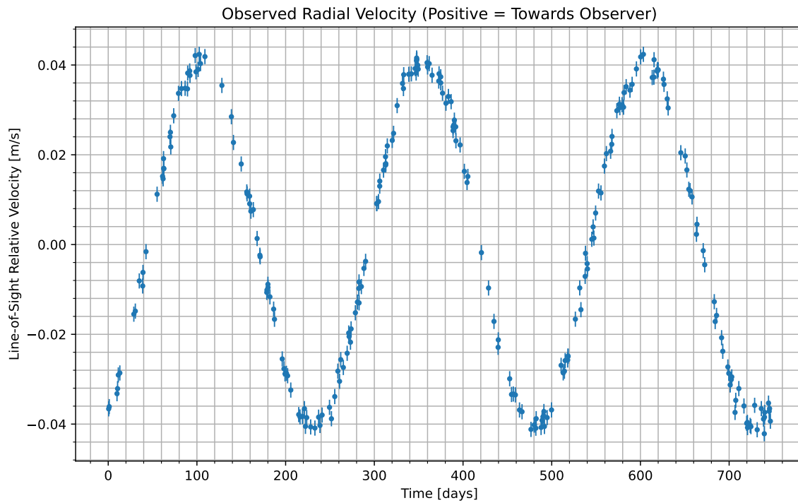
Figure 1: We have isolated the radial velocity of the host star due to the candidate planet. Data begins at UTC 2078-11-05/23:05. Positive values indicate the velocity at which the star is moving towards us; negative indicate the velocity at which it is moving away.
