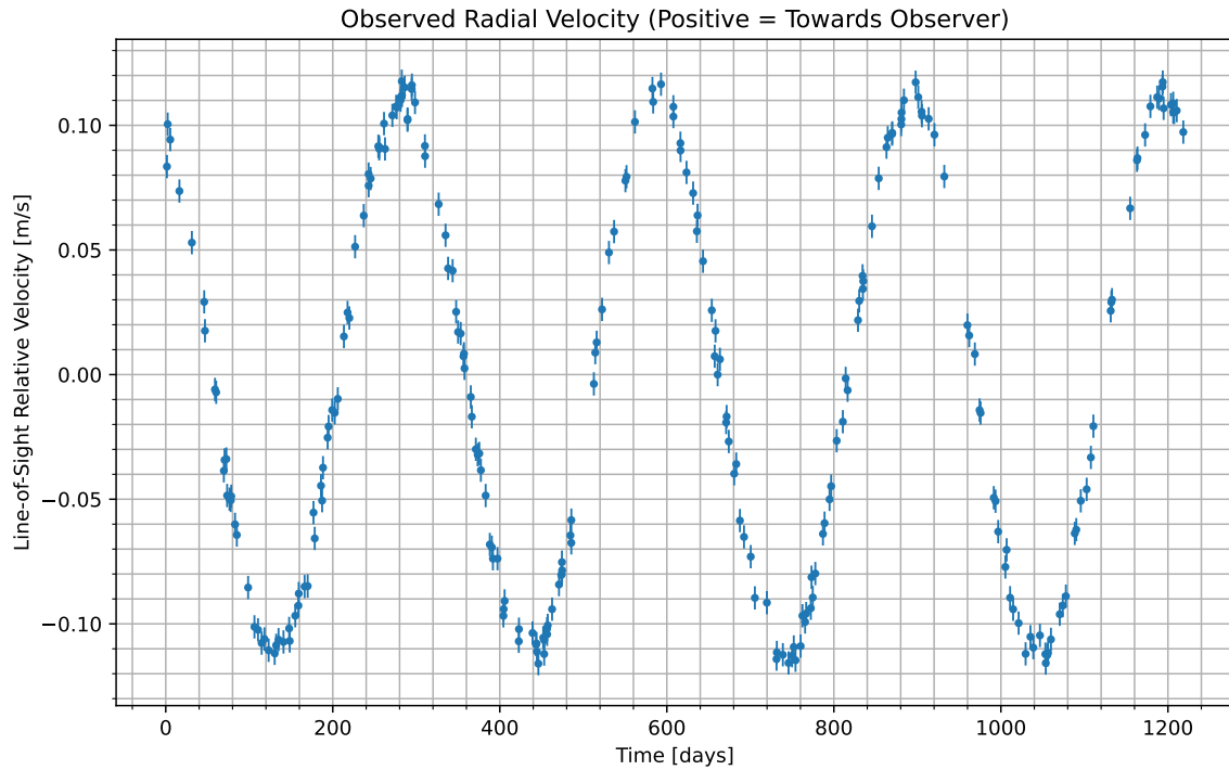
Figure 1: We have isolated the radial velocity of the host star due to the candidate planet. Data begins at UTC 2090-05-31/19:38. Positive values indicate the velocity at which the star is moving towards us; negative indicate the velocity at which it is moving away.
