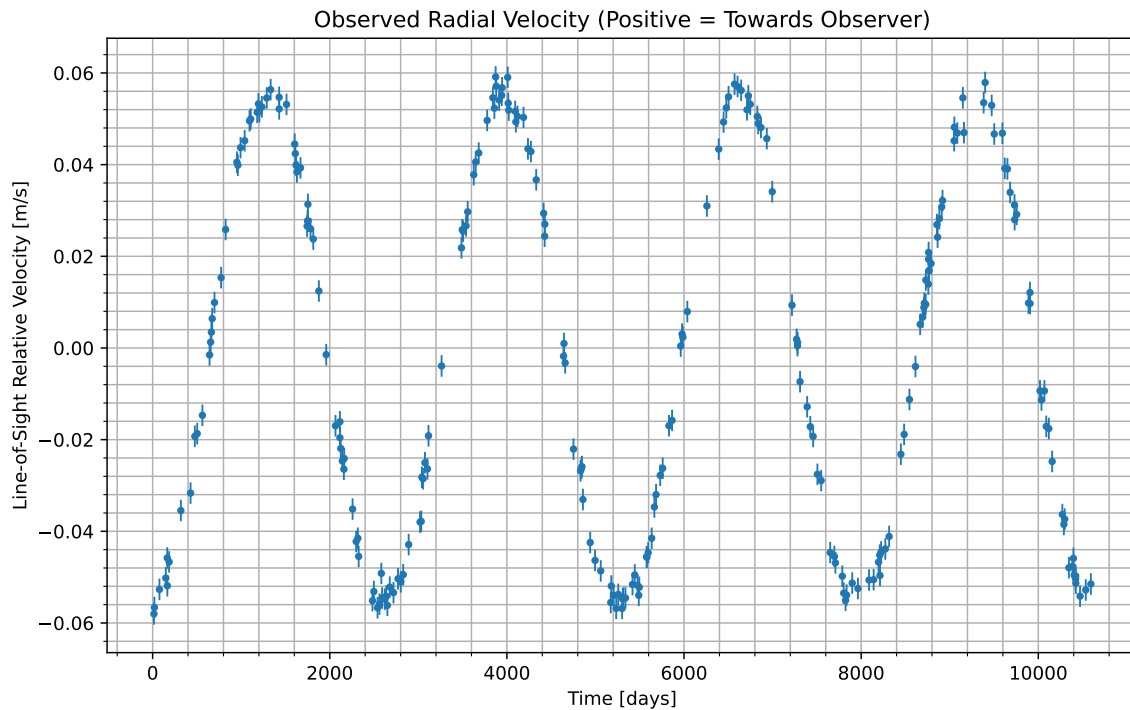
Figure 1: We have isolated the radial velocity of the host star due to the candidate planet. Data begins at UTC 2063-11-24/04:14. Positive values indicate the velocity at which the star is moving towards us; negative indicate the velocity at which it is moving away.
