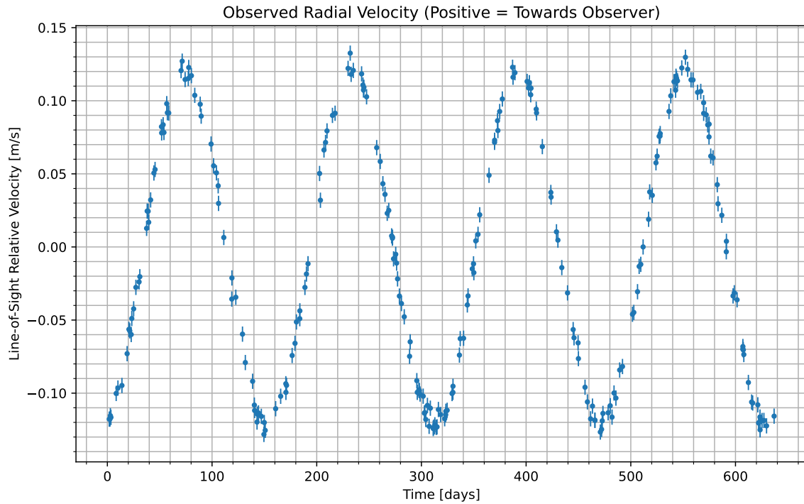
Figure 1: We have isolated the radial velocity of the host star due to the candidate planet. Data begins at UTC 2074-07-16/02:34. Positive values indicate the velocity at which the star is moving towards us; negative indicate the velocity at which it is moving away.
