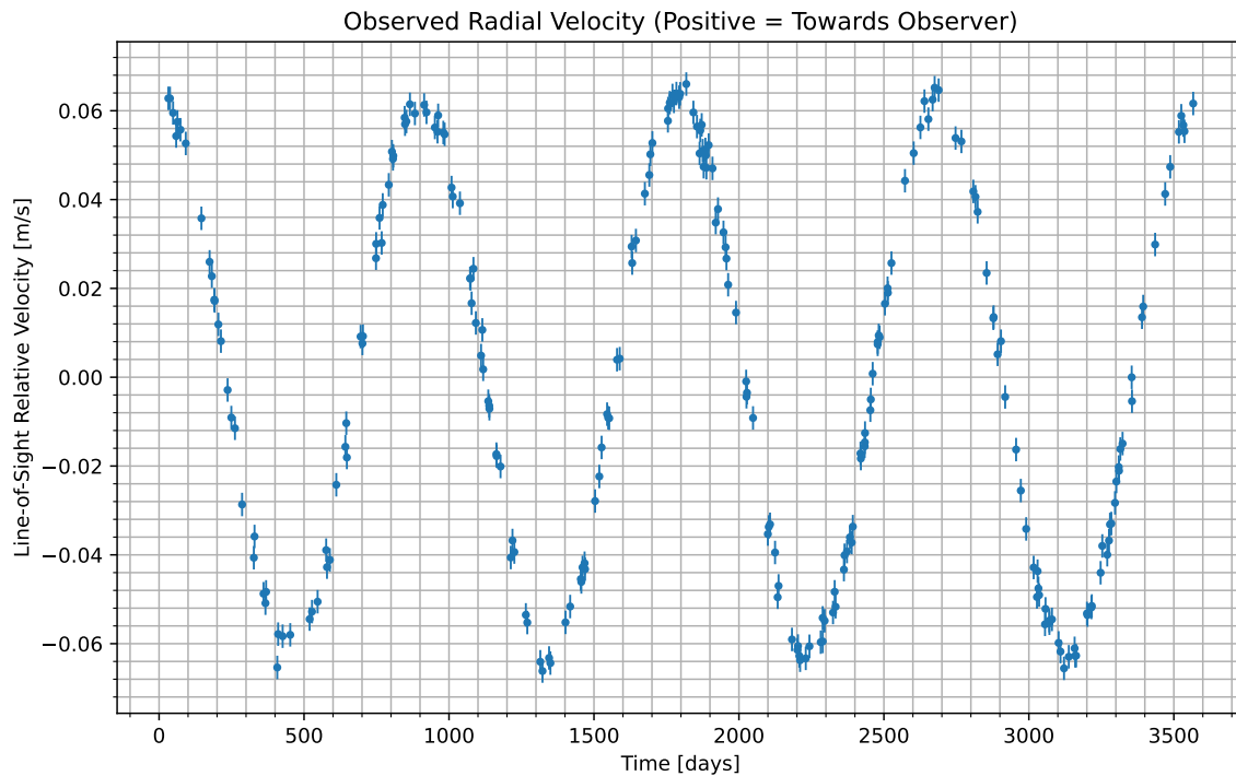
Figure 1: We have isolated the radial velocity of the host star due to the candidate planet. Data begins at UTC 2073-06-01/23:34. Positive values indicate the velocity at which the star is moving towards us; negative indicate the velocity at which it is moving away.
