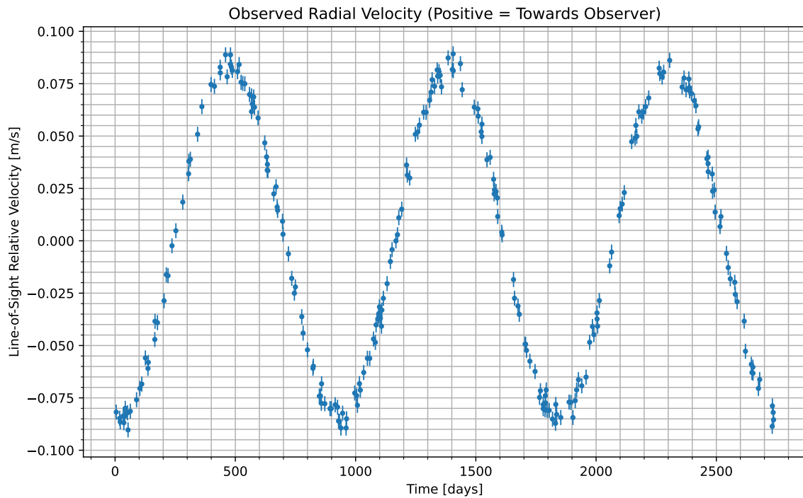
Figure 1: We have isolated the radial velocity of the host star due to the candidate planet. Data begins at UTC 2077-01-17/00:20. Positive values indicate the velocity at which the star is moving towards us; negative indicate the velocity at which it is moving away.
