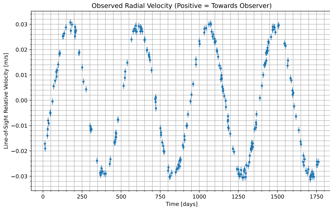
Figure 1: We have isolated the radial velocity of the host star due to the candidate planet. Data begins at UTC 2093-08-12/16:28. Positive values indicate the velocity at which the star is moving towards us; negative indicate the velocity at which it is moving away.
